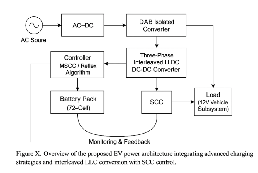
Fig 1: Overall architecture of the proposed EV power system, integrating MSCC-based intelligent charging control with a GaN-based interleaved LLC converter and SCC-assisted current balancing.
