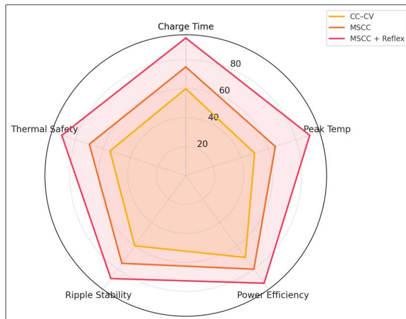
Fig 9: Comparative radar chart illustrating five key performance indicators across charging strategies. MSCC + Reflex consistently scores higher in efficiency, stability, and thermal safety, highlighting its superiority for EV battery management.
