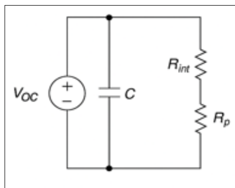
Fig 3: The venim Equivalent Circuit Model Of The Battery
