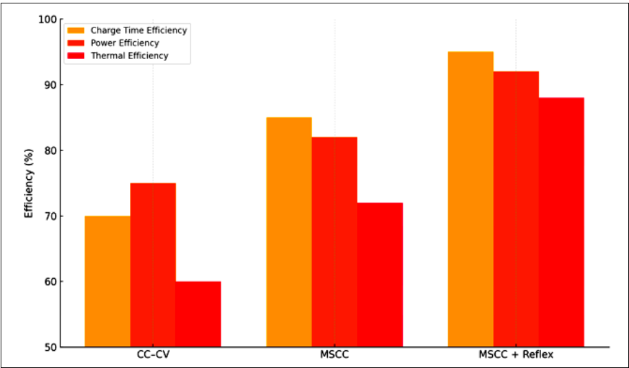
Fig 8: Efficiency comparison across charging strategies. MSCC + Reflex outperforms both CC-CV and MSCC methods in charge time, power delivery, and thermal regulation, aligning with trends reported in recent literature [22-29]
