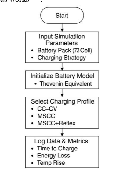
Fig 2: Flowchart of the simulation procedure illustrating the control logic and sequence for executing CC-CV, MSCC, and MSCC+Reflex charging strategies under MATLAB-based modeling.
