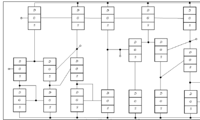
Fig 1: The considered the comparator [4]
