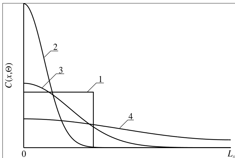
Fig 4a: Distributions of concentration of infused dopant in depth of hetero structure from Fig. 1 for different values of annealing time (curves 2-4) and idealized step-wise approximation (curve 1). Increasing of number of curve corresponds to increasing of annealing time
