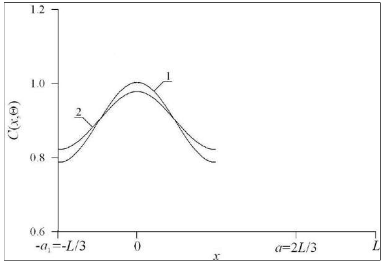
Fig 3a: Distributions of concentration of dopant, infused in average section of epitaxial layer of hetero structure from Figs. 1 in direction parallel to interface between epitaxial layer and substrate of hetero structure. Difference between values of dopant diffusion coefficients increases with increasing of number of curves. Value of dopant diffusion coefficient in this section is smaller, than value of dopant diffusion coefficient in nearest sections
