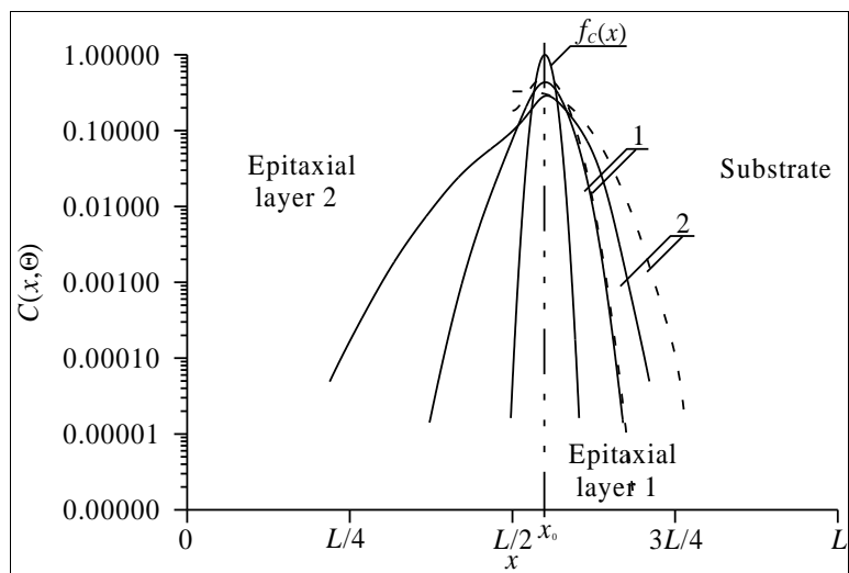
Fig 3b: Calculated distributions of implanted dopant in epitaxial layers of hetero structure. Solid lines are spatial distributions of implanted dopant in system of two epitaxial layers. Dashed lines are spatial distributions of implanted dopant in one epitaxial layer. Annealing time increases with increasing of number of curves
