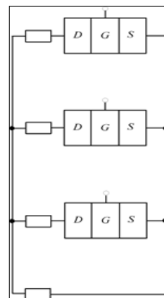
Fig 1(a): Structure of the considered amplifier [24]
